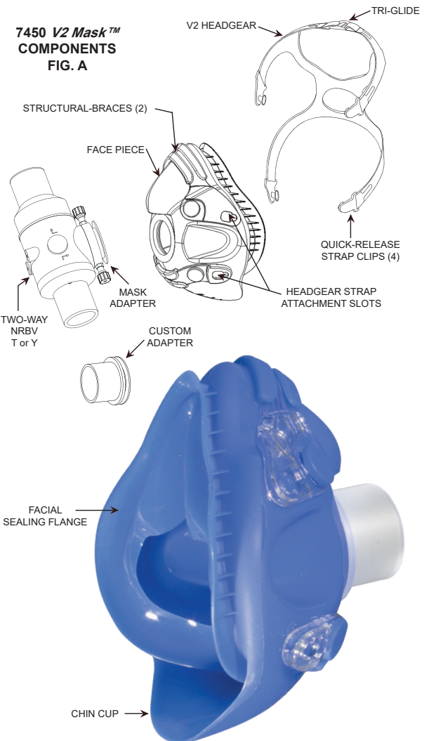
Oro-Nasal 7450 V2 Mask™ with Headgear and 2730 2-Way Y-Shape™ Non-Rebreathing Valve
